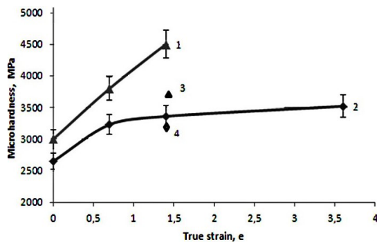
Fig. 1- Microhardness dependence on true strain with EPR ( j = 100 \text{ A/mm}^2 ): (1) Ti_{49.2}Ni_{50.8} (2) Ti_{50.0}Ni_{50.0} (3) Ti_{49.2}Ni_{50.8} + annealing at 500 °C, (4) Ti_{50.0}Ni_{50.0} + annealing at 500 °C.
