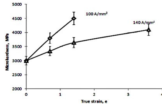
Fig. 2- Influence of current density on strain hardening in Ti_{49.2}Ni_{50.8} alloy.
