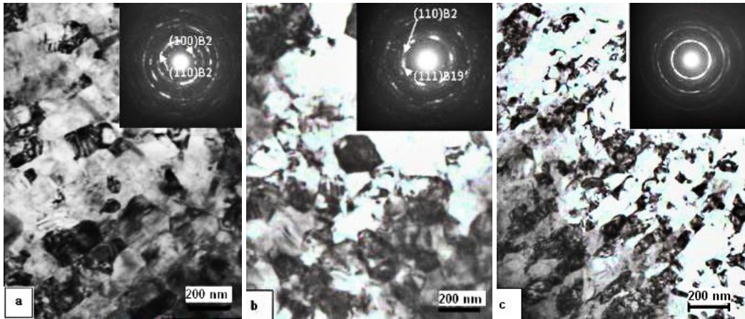
Fig. 3- Microstructures and SAEDP of alloys after EPR and annealing: (a) Ti_{49.2}Ni_{50.8} , e = 1.2 + annealing at 500 °C for 1 hour; (b) Ti_{50.0}Ni_{50.0} , e = 1.4 + annealing at 500 °C for 1 hour; (c) Ti_{50.0}Ni_{50.0} , e = 1.4 + annealing at 450 °C for 1 hour.
