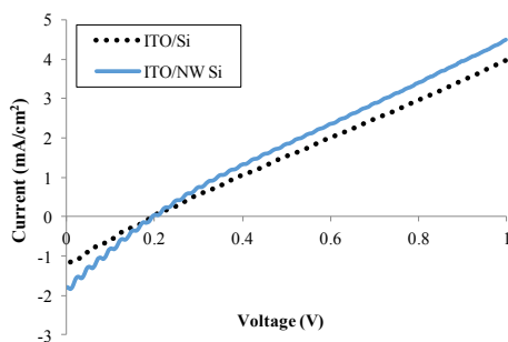
Fig. 6- I-V characteristics of Ag/ITO/Si Schottky diode, illuminated with AM1.5 standardized light, with and without Si NWs
