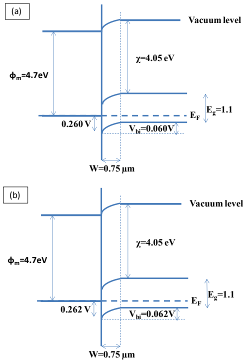
Fig. 2- Band energy diagrams for Schottky contact between ITO on (a) Si and (b) NW/Si substrates.
