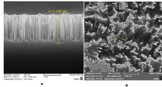
Fig. 3- (a) SEM image of Si NWs cross-section. (b) surface morphology of Si NWs
