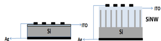
Fig. 1- Schematic diagram of Ag/ITO/Si Schottky solar cell, with and without Si NWs.
