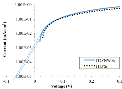
Fig. 5- I-V characteristics of Ag/ITO/Si Schottky diode, in dark condition, with and without Si NWs.
