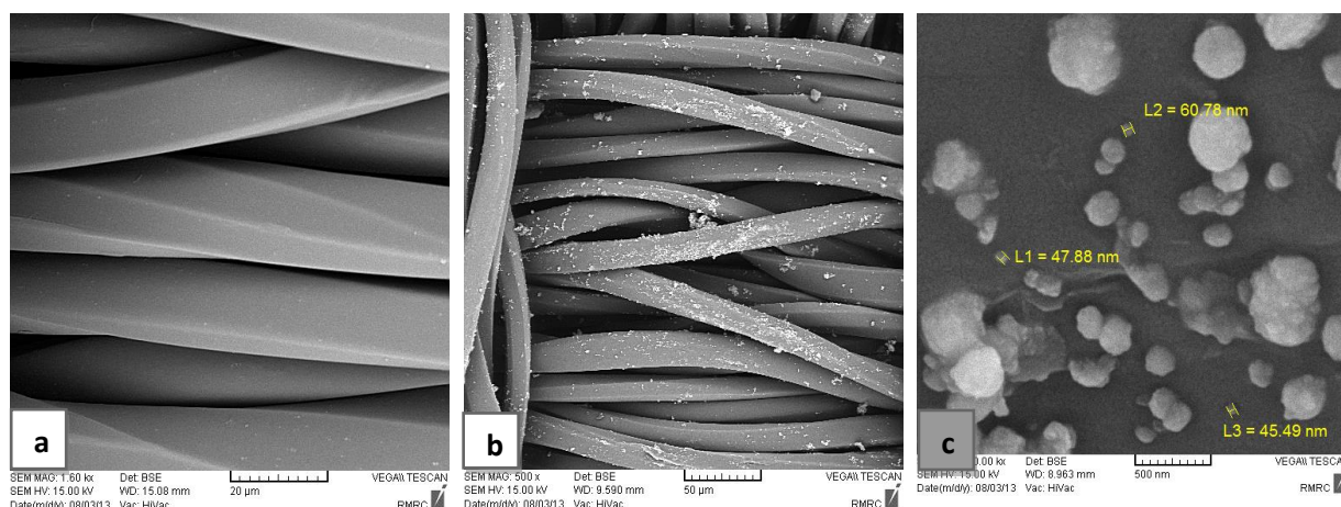
Fig. 3. SEM of the a) untreated and b,c) treated polyester fabric with ZnO nano particleu'
