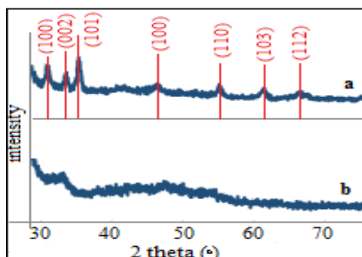
Fig. 2. XRD pattern of the a) treated and b) untreated polyester fabric with ZnO nano particles
